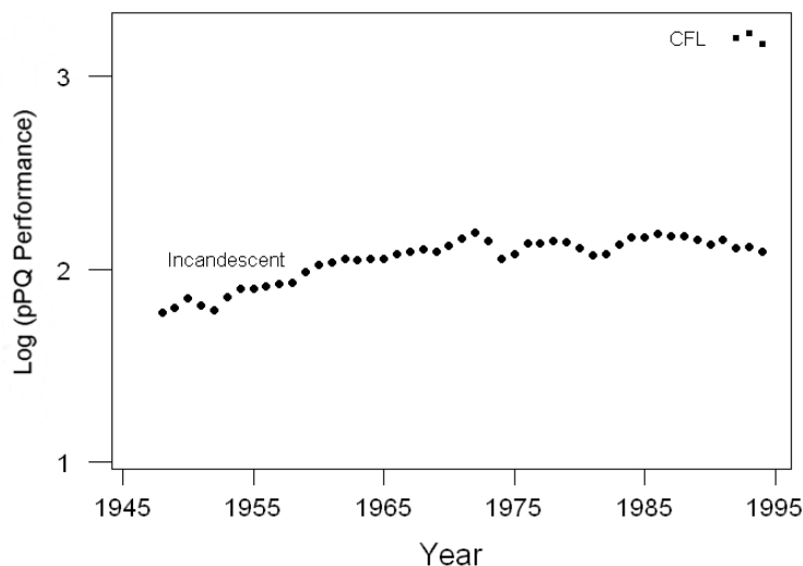
Figure 30 – Performance of Incandescent and Compact Fluorescent
