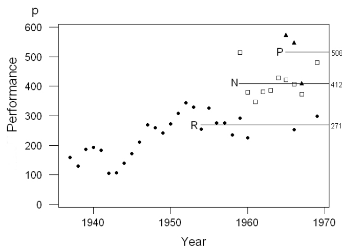
Figure 9 – Tire Cord Performance calculated from pPQ
