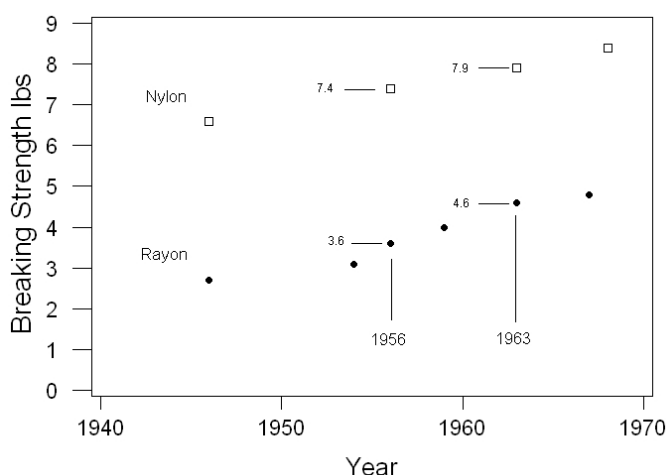
Figure 6 – Tire cord strength development
