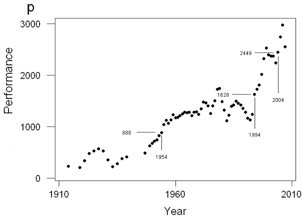
Figure 11 – Performance of Portland Cement
